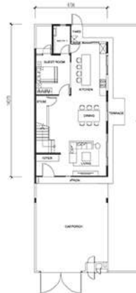
Ground Floor
